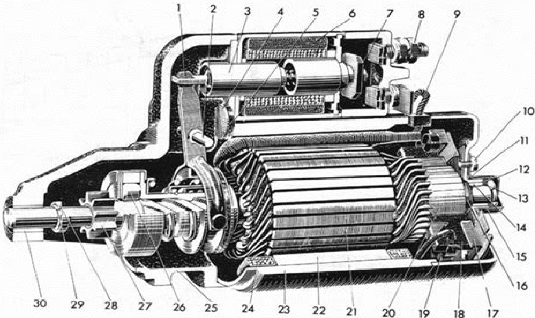
Fig. 10.10. Cut-away view of starter motor (Sec. 11)
