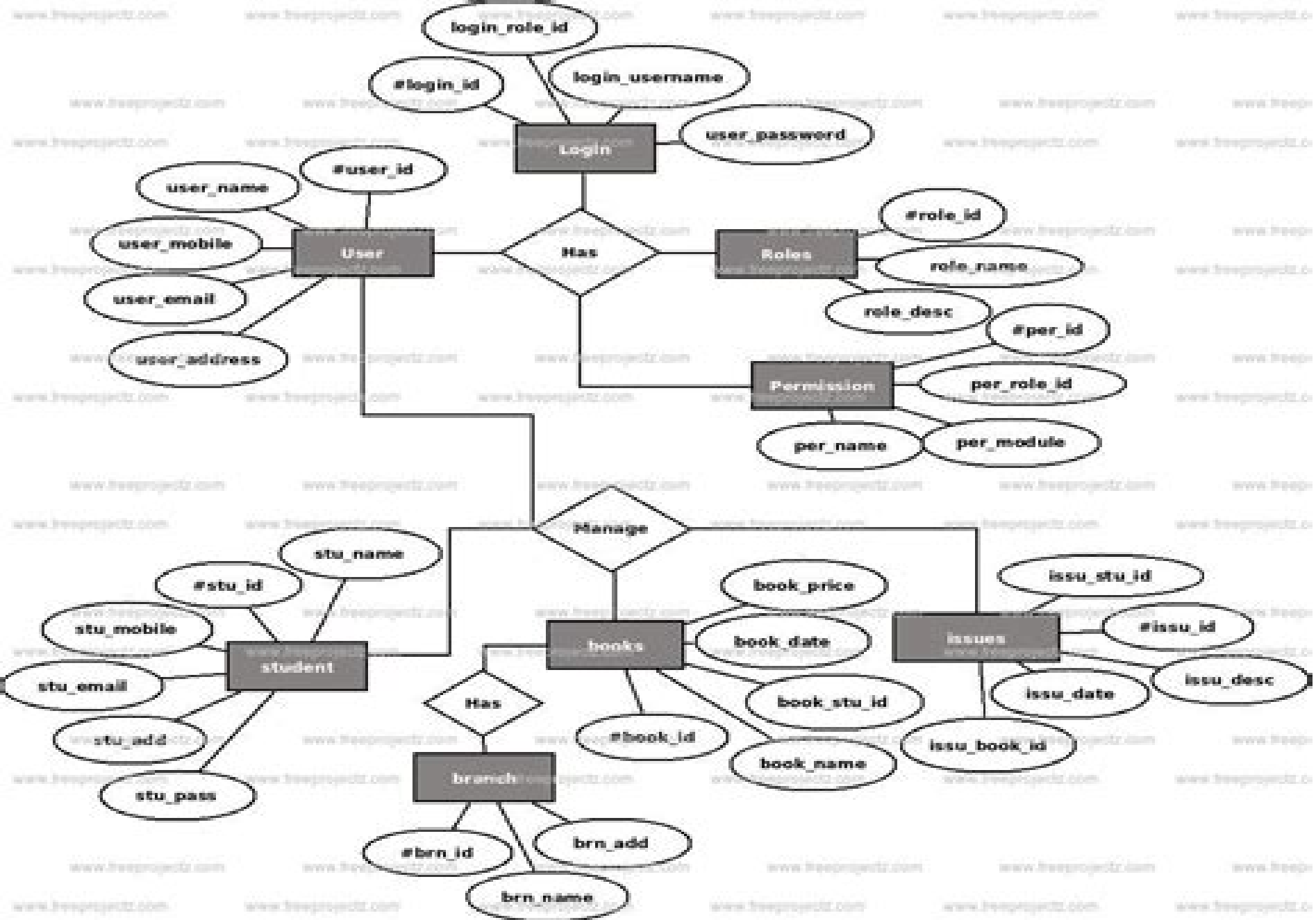
ER Diagram For College Management System
