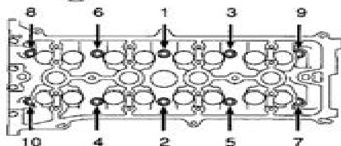
Cylinder Head Bolt Torque Sequence
