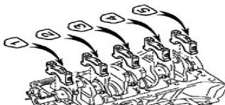
Main Bearing Cap Bolt Torque Sequence
