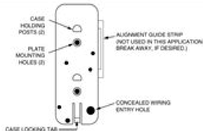
Diagram 1: MOUNTING PLATE
