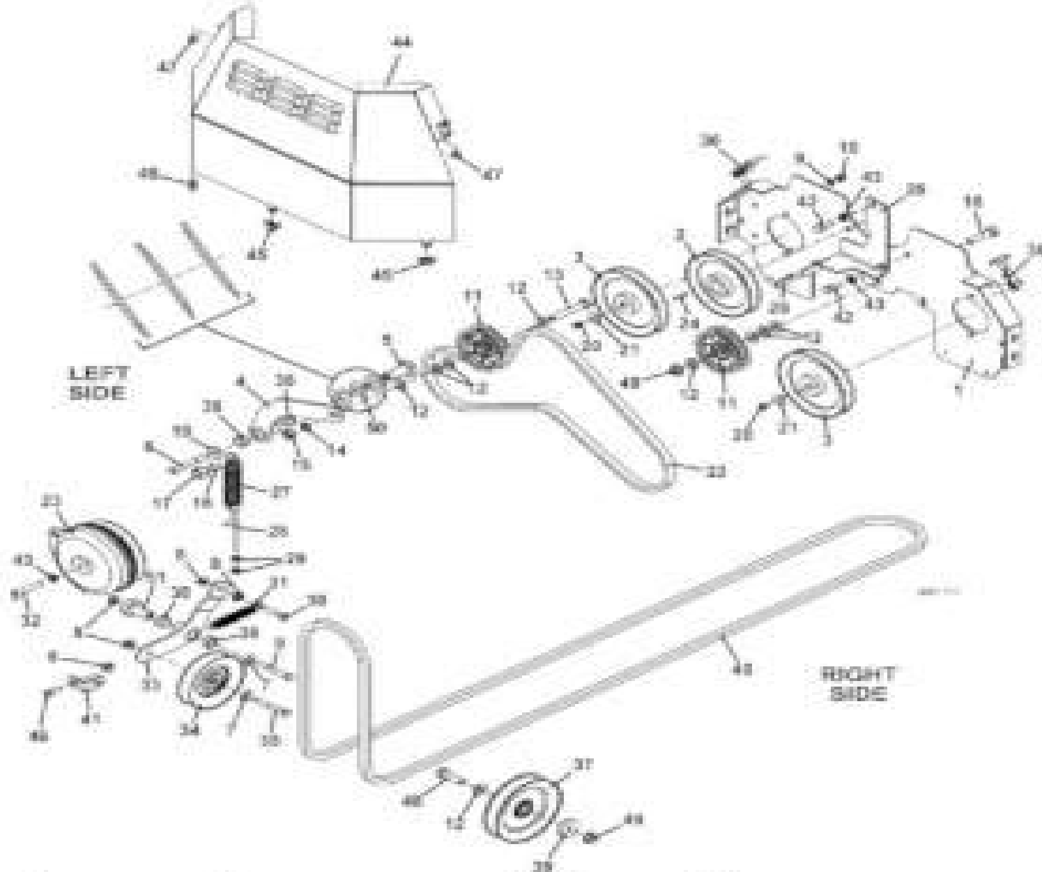
Drive Assembly diagram 1
