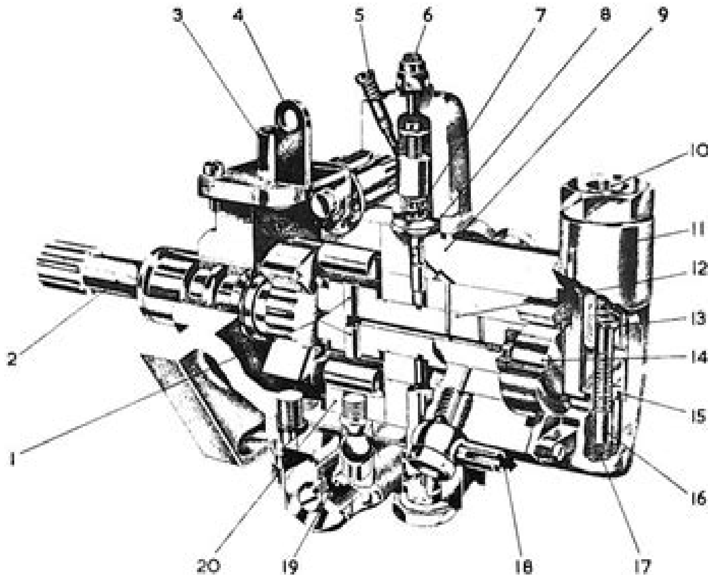
DPA pump with hydraulic governor and automatic advance device
