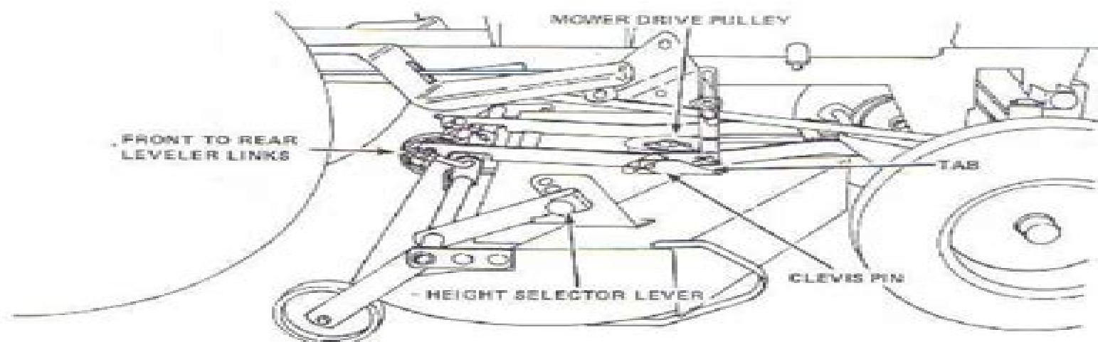
FIGURE 17 MOUNTING THE L44 MOWER DECK
