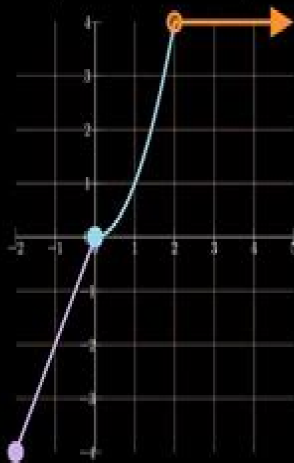
Graph of f(x)
