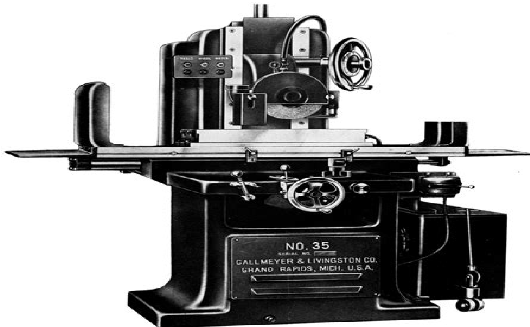
No. 35 Grand Rapids Hydraulic Surface Grinder
