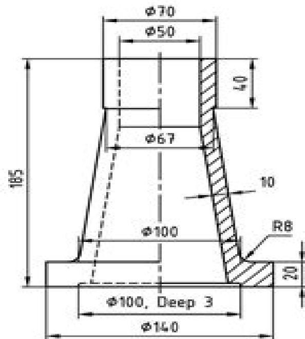
BODY (CAST IRON )
