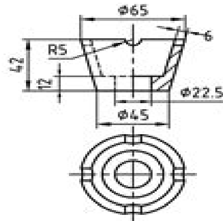
CUP (CAST STEEL)
