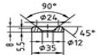
SPECIAL WASHER (MILD STEEL)
