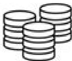
Multiple Oracles
