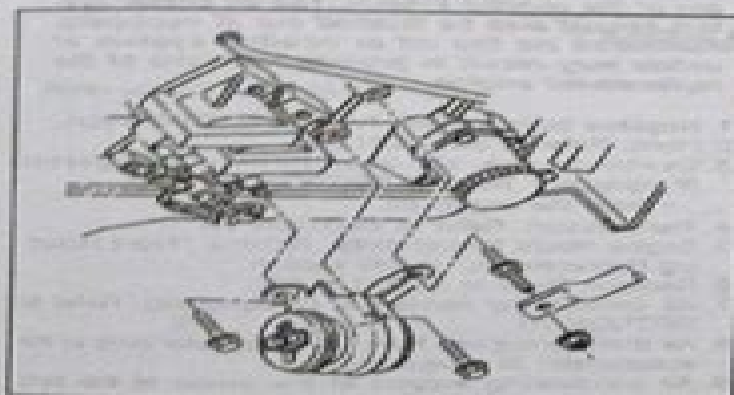
Figure 23—Front Engine Mount (Right Side)
