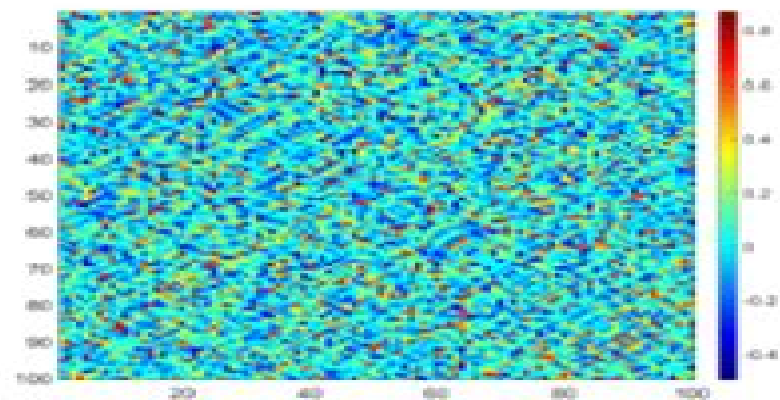
(b) A random weighted network/ graph
