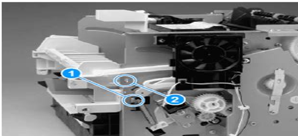
Figure 38. Removing the front guide assembly (2 of 3)
