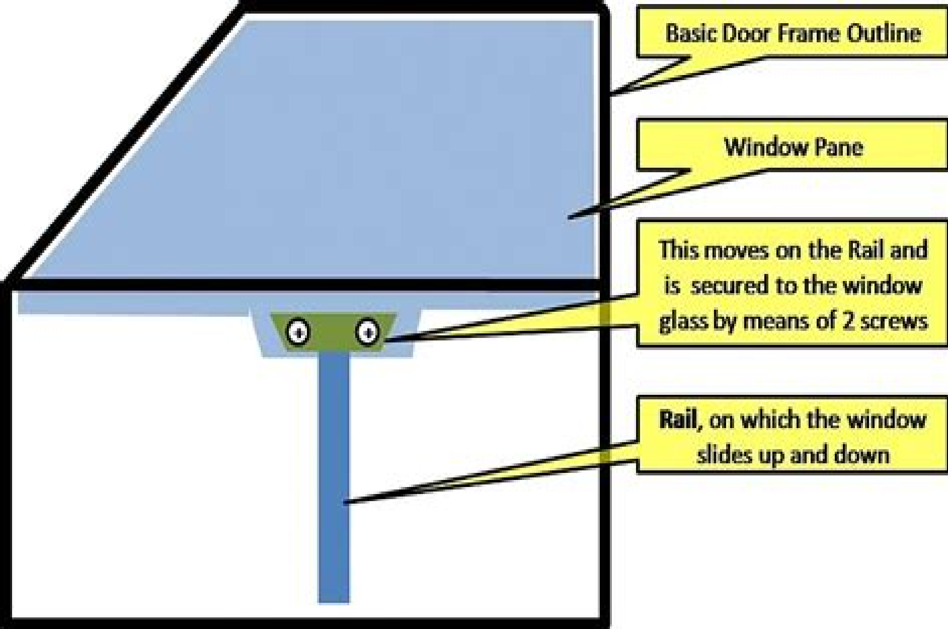
Fig A: When the window is rolled up
