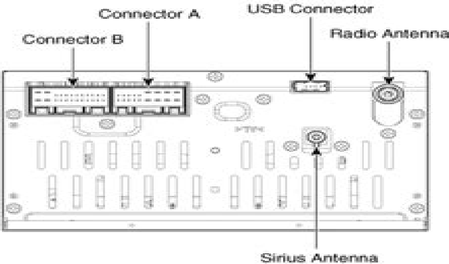
[Internal Amplifier]
