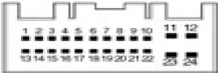
Connector B
