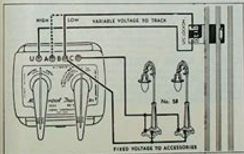
Figure 2—Track and Accessory Connection for "Multi-Control" Transformer.
