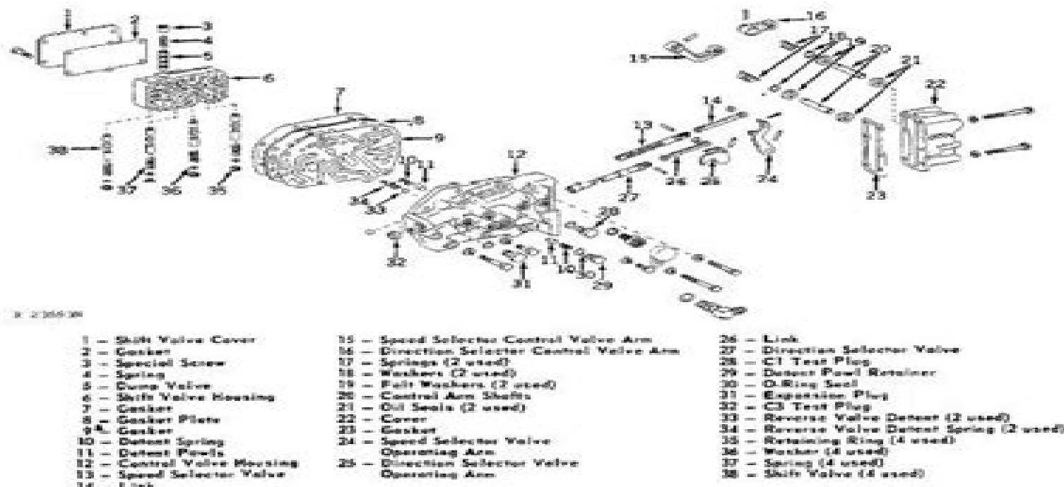
Fig. 16-Transmission Control Valve Parts
