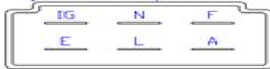
Pin lay-out of 6-pole connector
