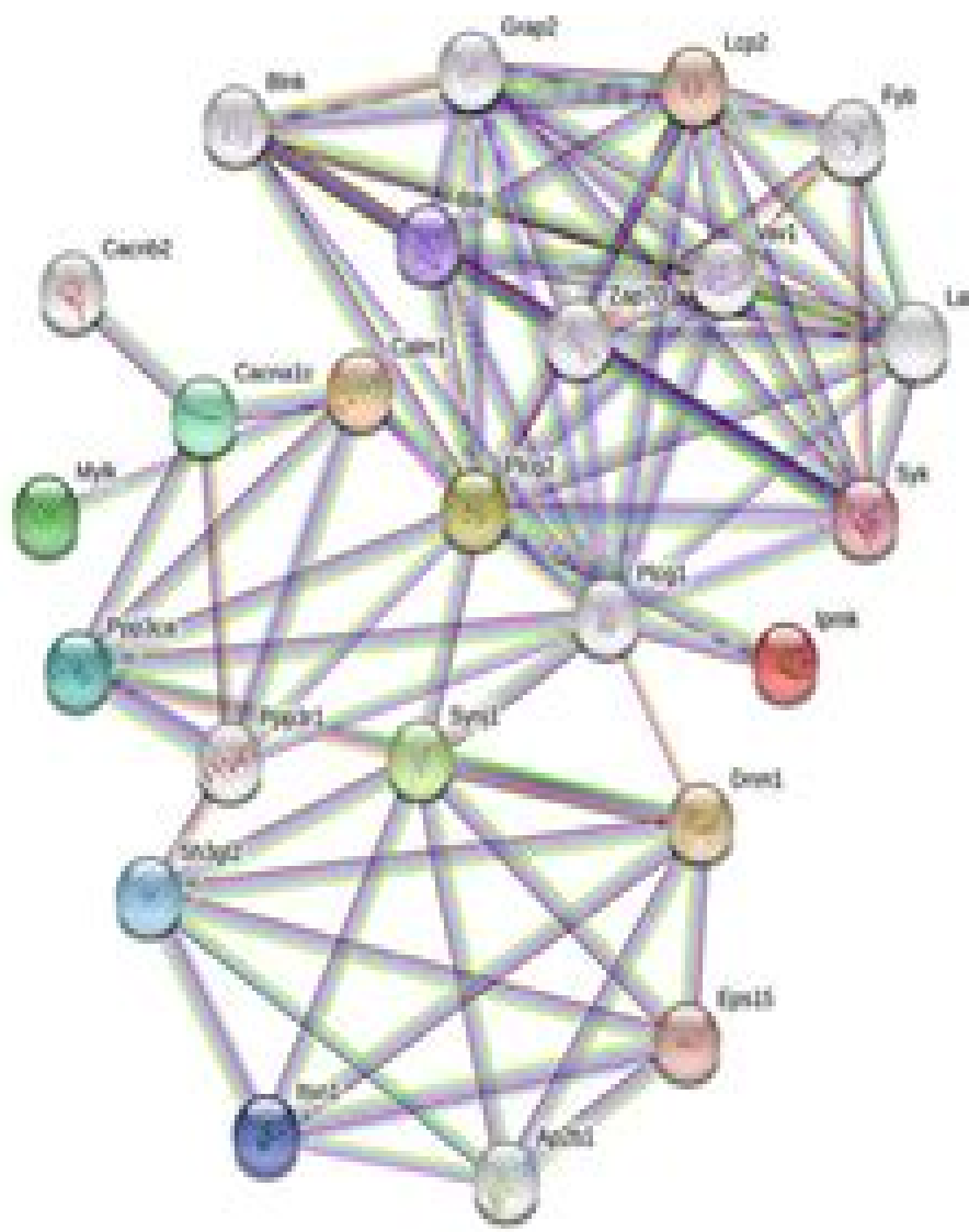
(A) Inositol Phosphate Metabolism pathway
