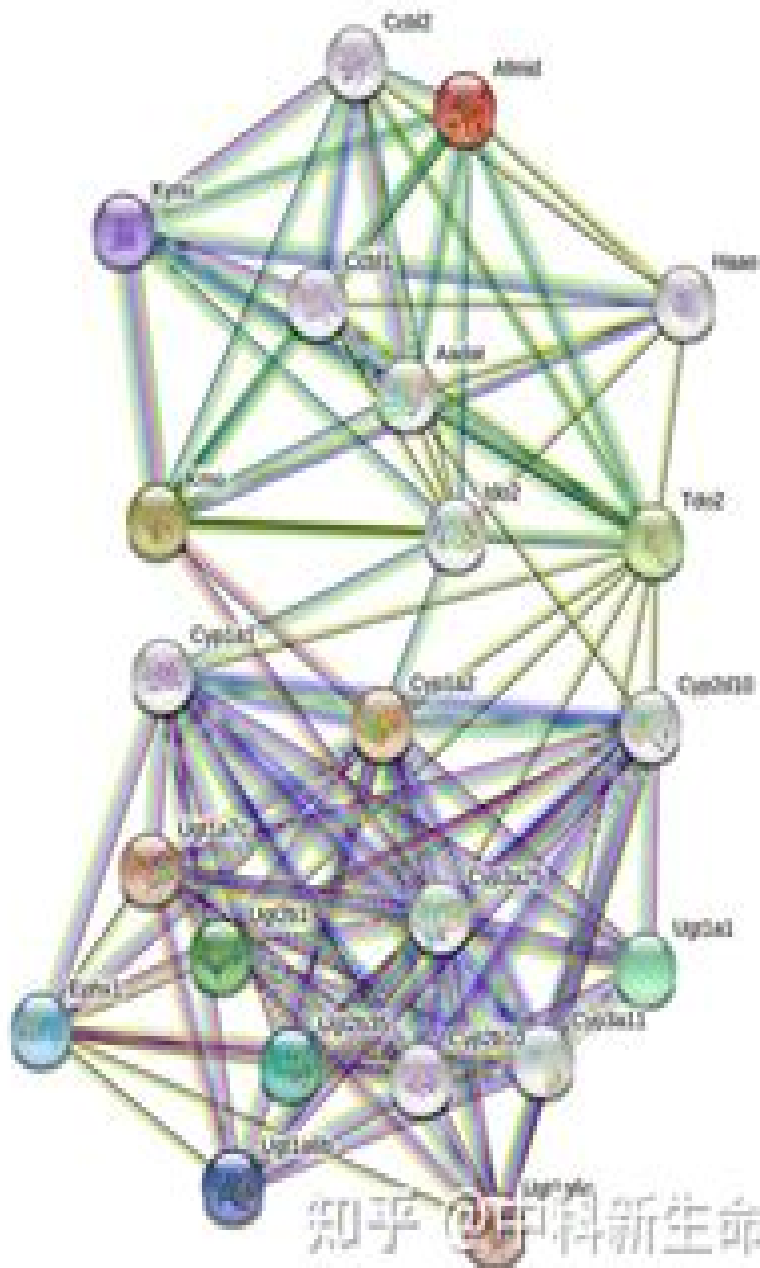
(B) Tryptophan metabolism
