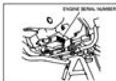
ENGINE SERIAL NUMBER The engine serial number is stamped on the lower left side of the cylinder.
