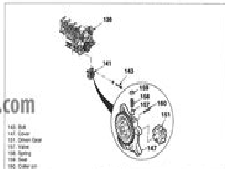
Figure 75: Oil Pump
