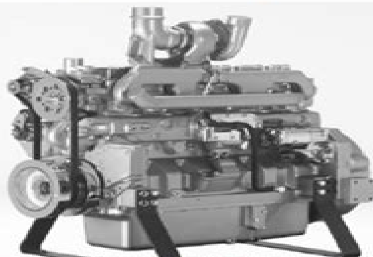
B.1 L Diesel Engines Left Front View (Engines 200,000— )
