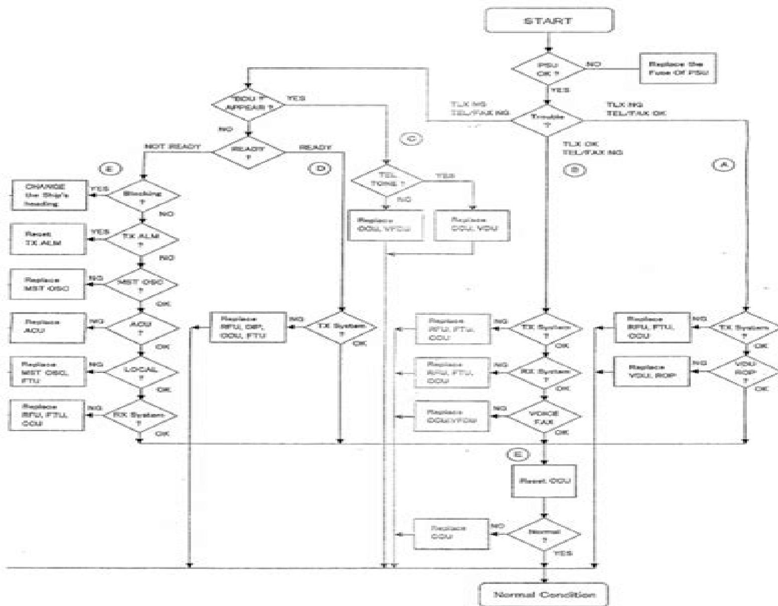
Fig. 1 JUE-310B TROUBLE SHOOTING GENERAL CHART
