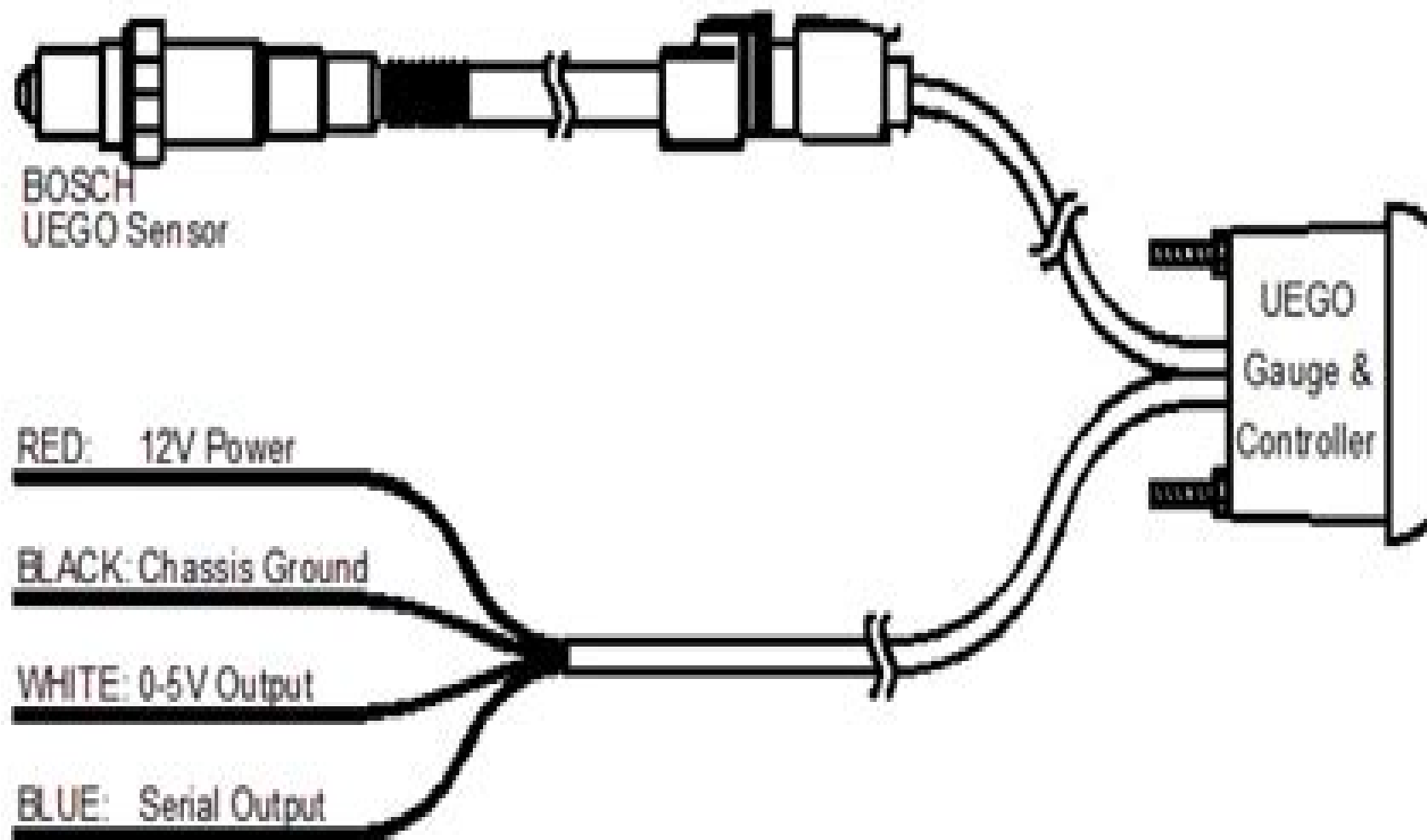
Figure 3. Gauge Installation Connections
