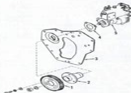
Fig. 13—Exploded view of injection pump drive gear drive.
