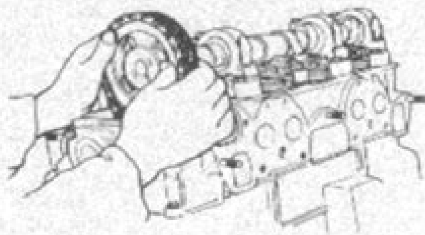
Fig. EM-14 Removing camshaft sprocket
