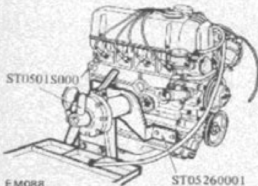
Fig. EM-11 Engine on engine stand
