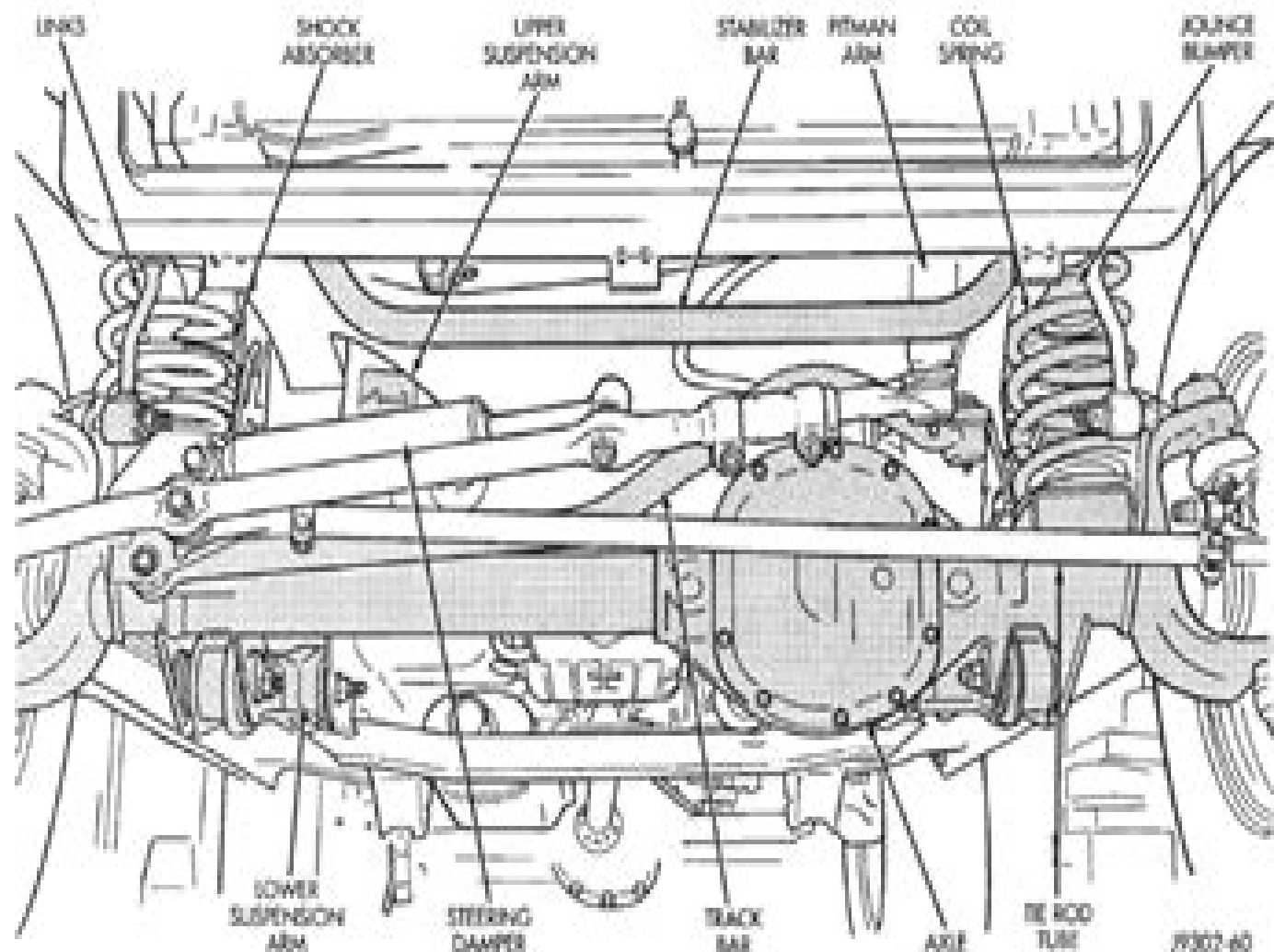
Fig. 1 Front Suspension
