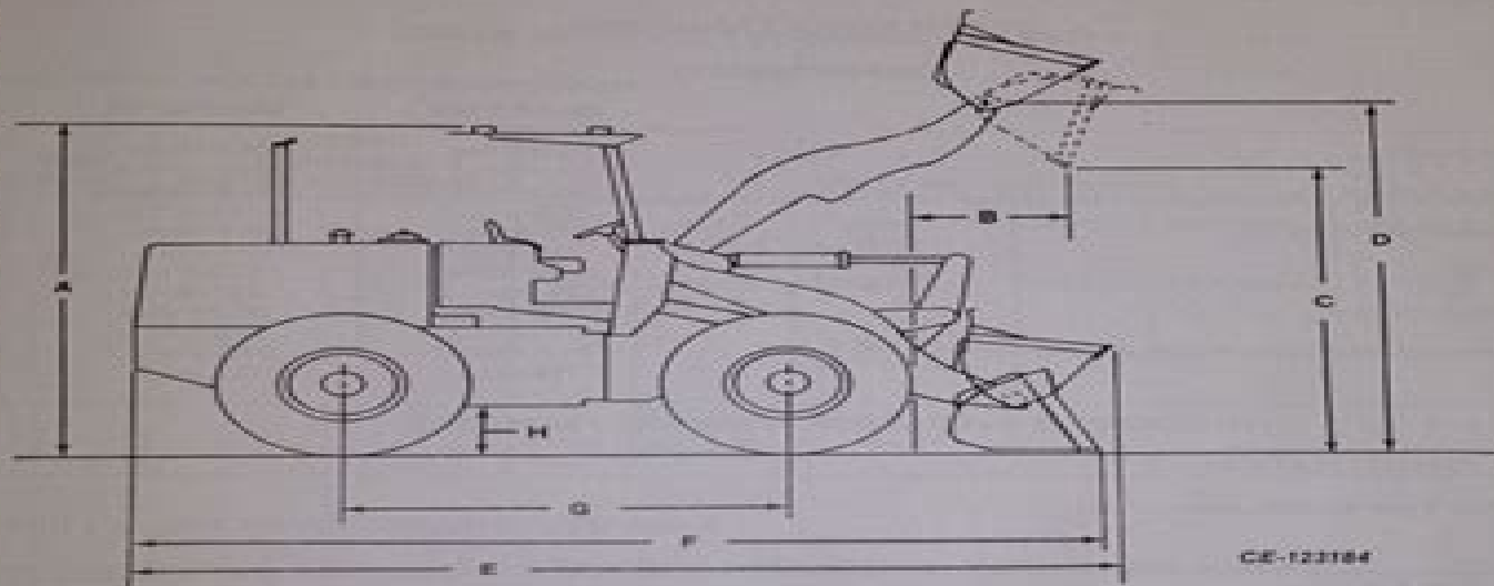
FIG. 1 — General Dimensions
