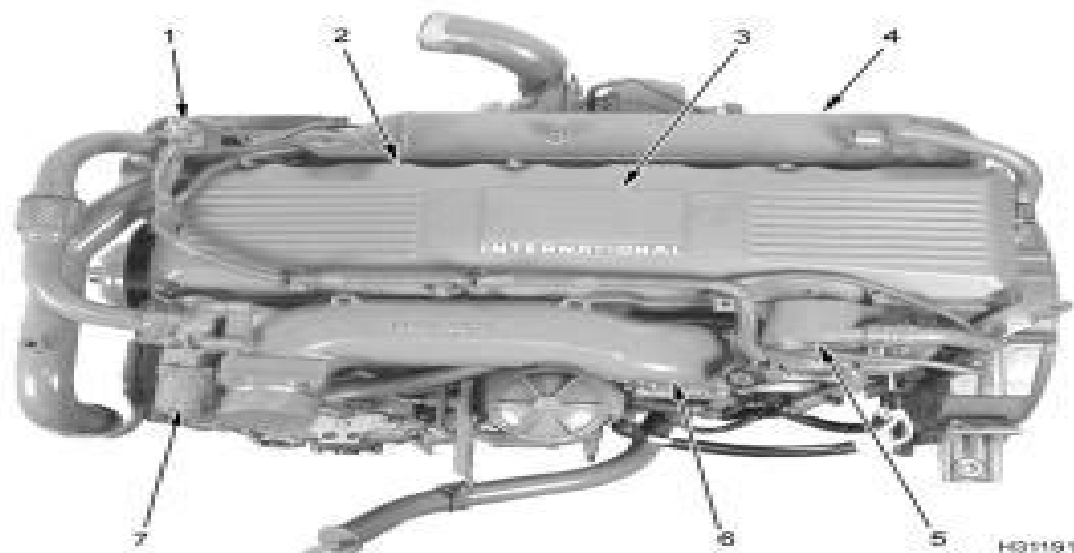
Figure 4 Component location – top
