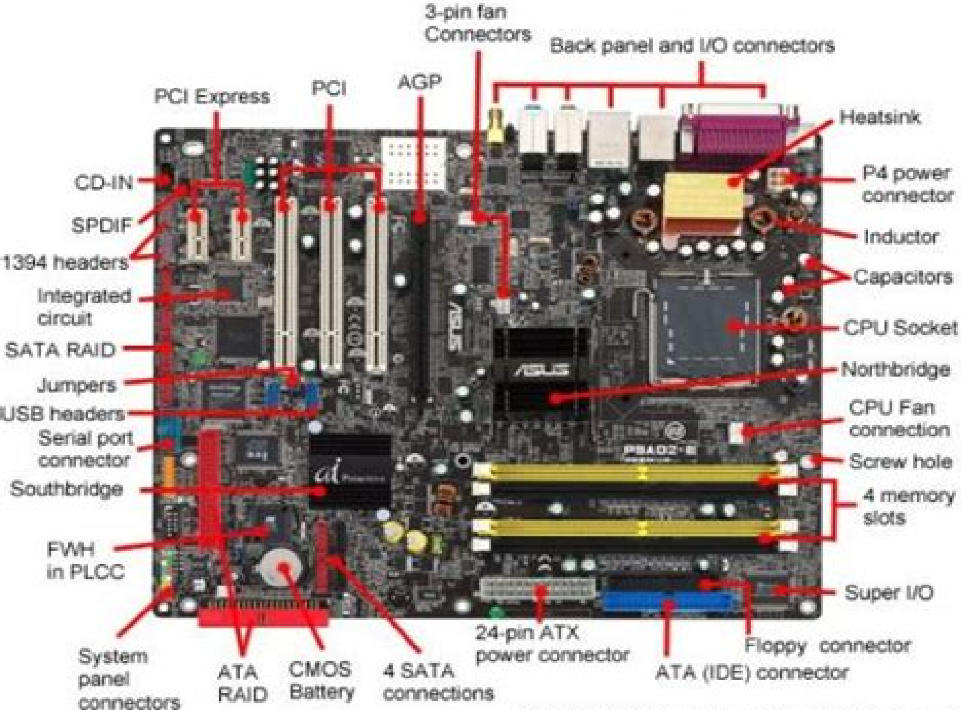
ASUS P5AD2-E Premium Motherboard
