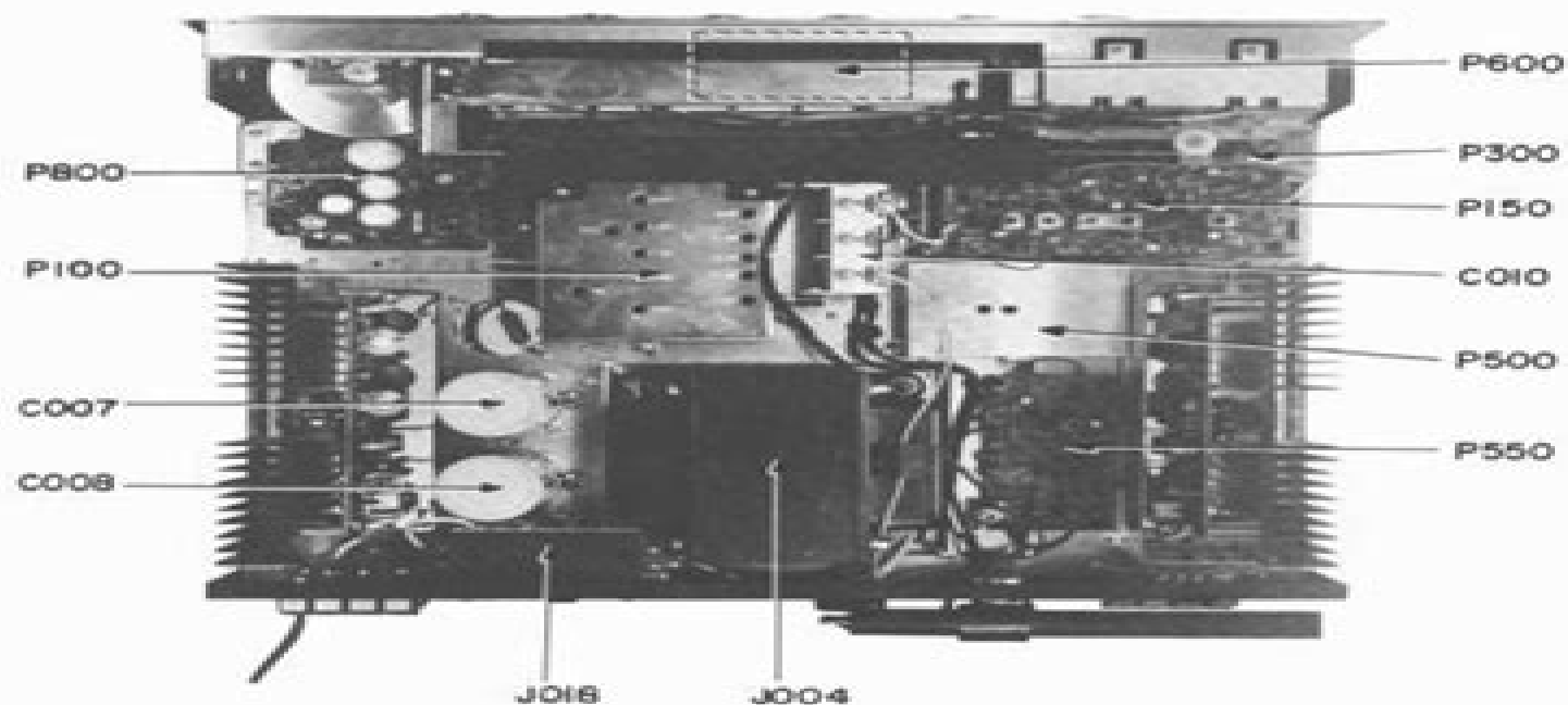
Figure 6. Main Chassis Component Locations (Top View)
