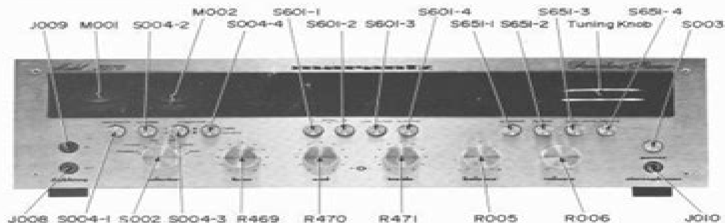
Figure 5. Front Panel Adjustment and Component Locations
