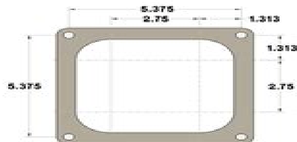
HOLLEY 4500 (DOMINATOR)
