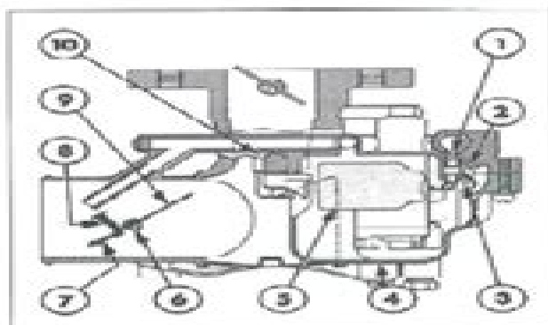
Figure 2 Fuel and Choke Systems
