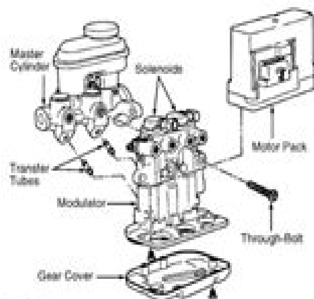
Fig. 4. Identifying ABS Modulator/Motor Pack & Master Cylinder Assembly Components Courtesy of GENERAL MOTORS CORP.
