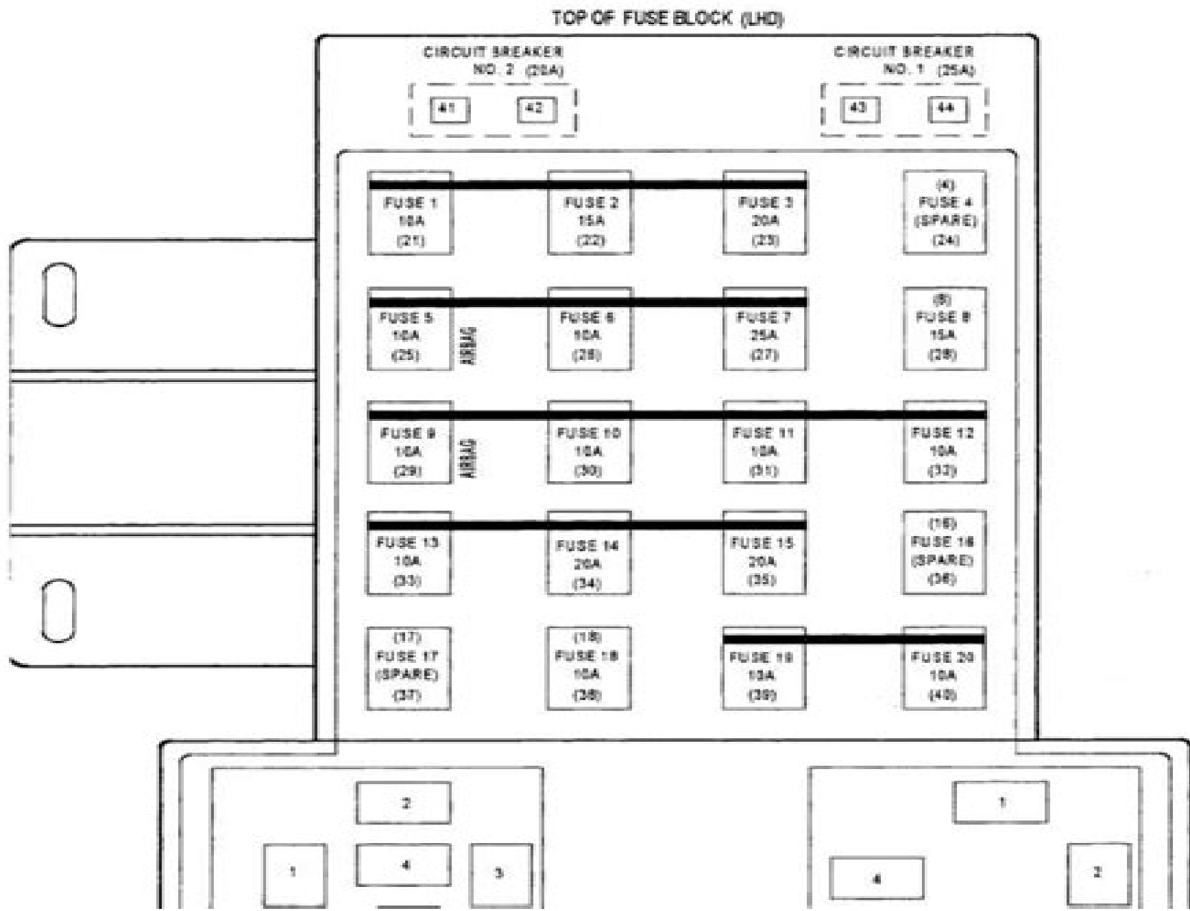
Fig 4: Identifying Fuse Block Components
