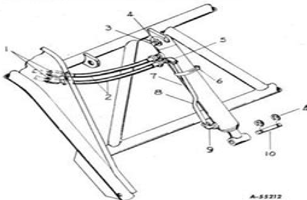
FIGURE 4, SINGLE ATTACHMENT CYLINDER CONNECTIONS
