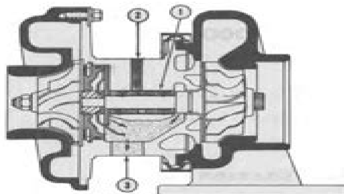
Figure 2 Turbocharger Lubrication
