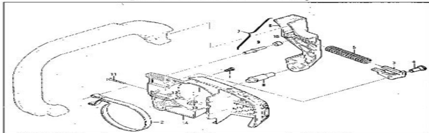
Figure 5. CHAIN BRAKE Assembly.
