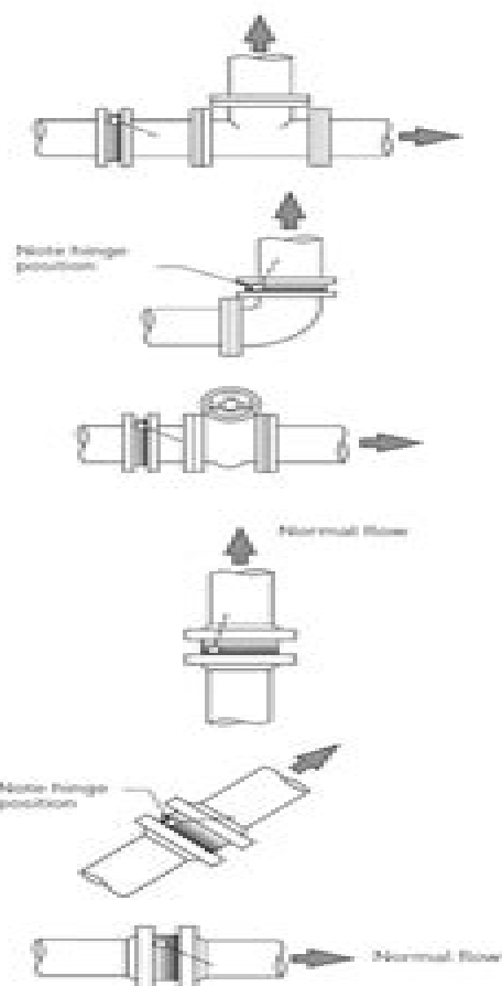
FIGURE 1. Installation positions, elevation view
