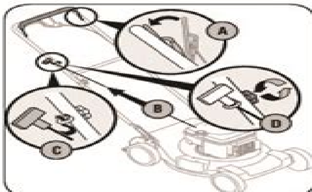
Figure 3-3: Pull recoil starter through rope guide and tighten.
