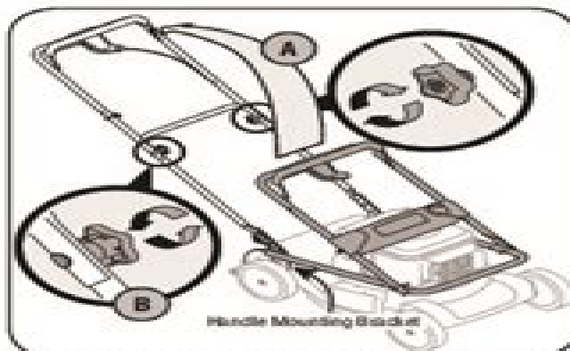
Figure 3-1: Unfold handle and tighten hardware.
