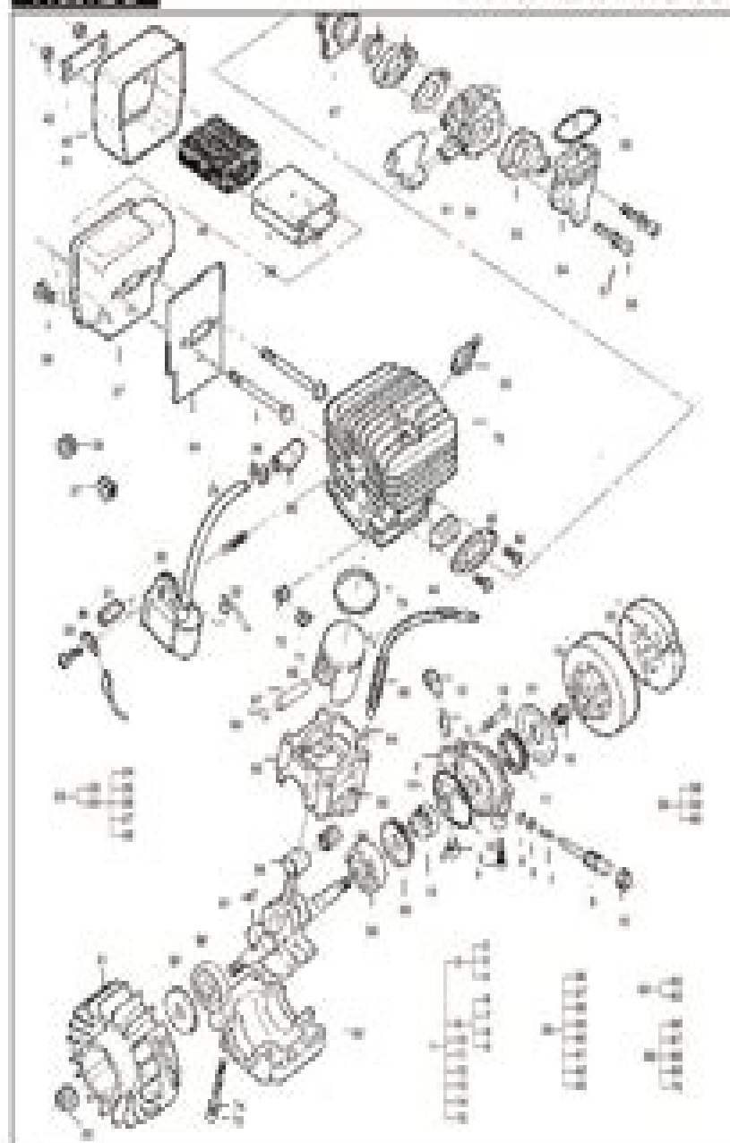
POWERHEAD ASSEMBLY
