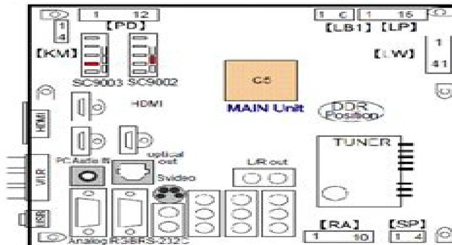
Destination ID connector locations
