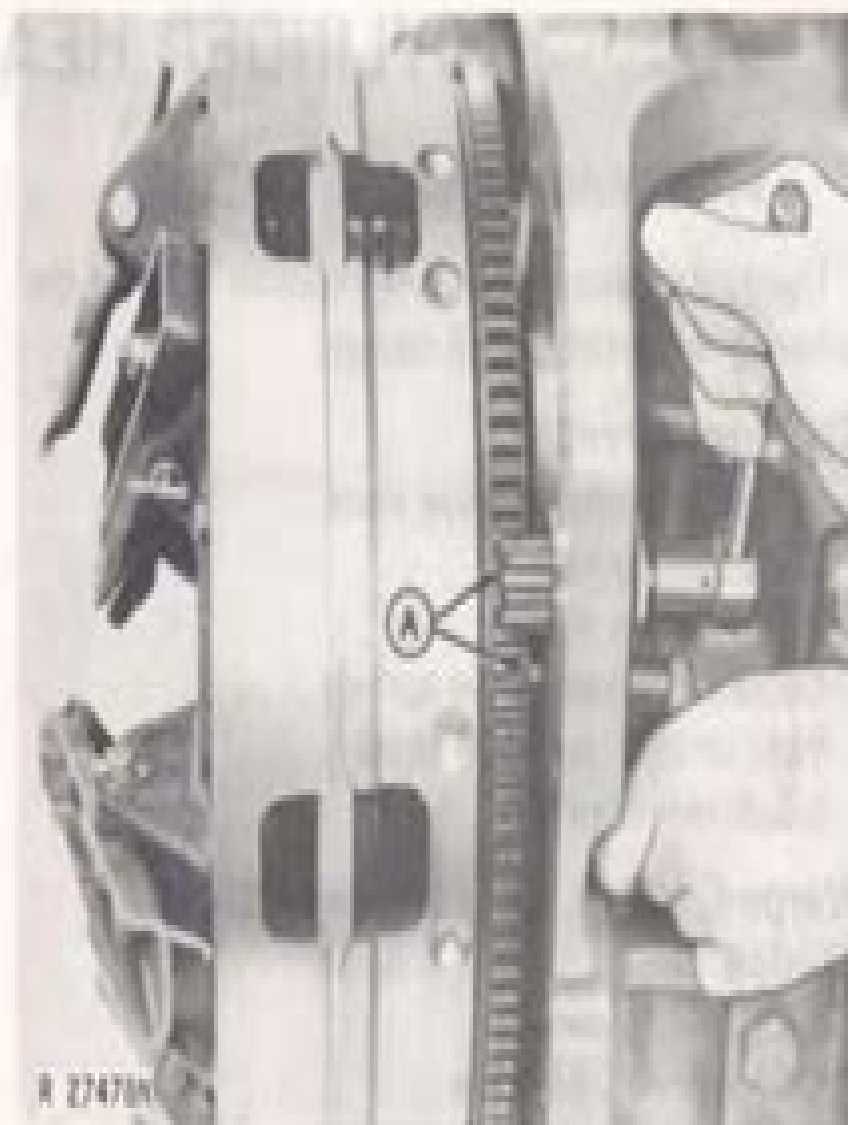
Fig. 3-Setting "TDC"
