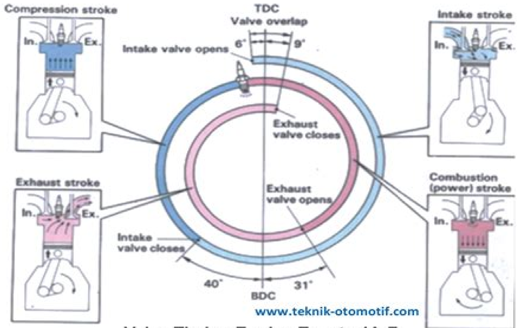
Valve Timing Engine Toyota 4A-F
