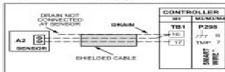
Figure 1. Sensor Wiring
