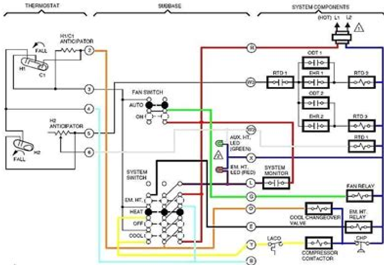
Fig. 6. Internal schematic and typical wiring diagram for Y594R1243 (T874R1152/Q674L1207).
