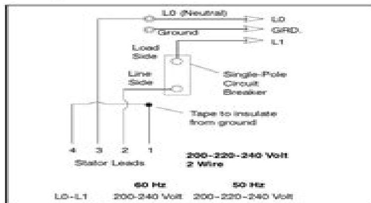
Figure 8-4 200-220-240-Volt, 2-Wire Configuration
