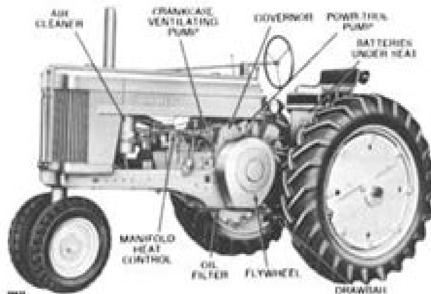
John Deere Model "60" Tractor—Flywheel Side
