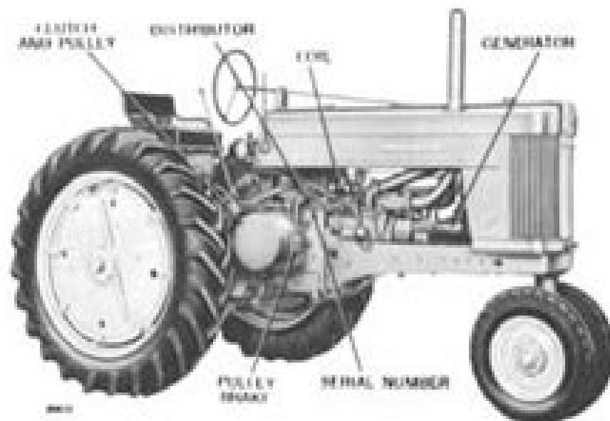
John Deere Model "60" Tractor—Pulley Side
