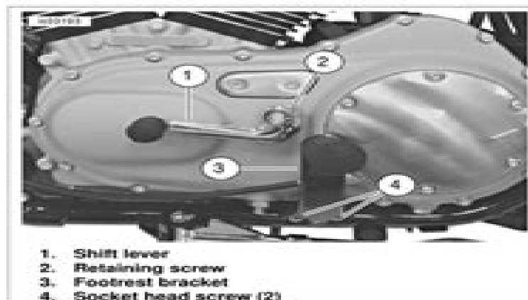
Figure 1. Remove Shift Lever and Footrest
