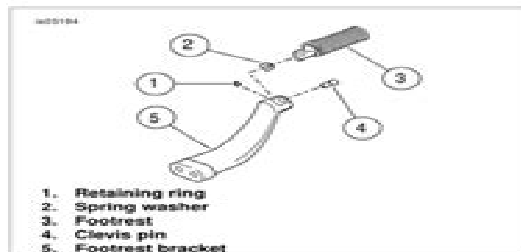
Figure 2. Remove Left Footrest - All Models except XL883L and XL1200N
